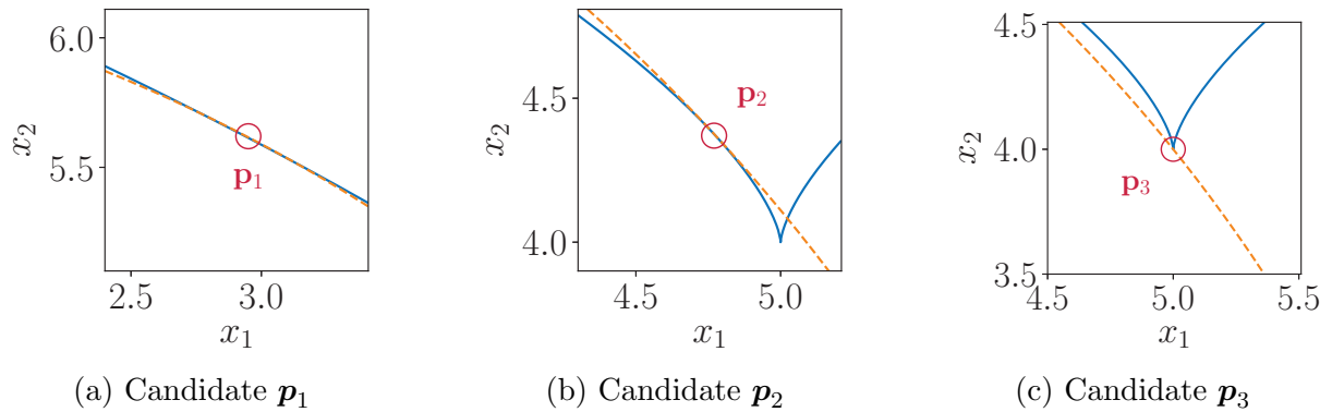
Figure 3: Candidates (circles) in feasible set (solid lines) and corresponding contours of cost function (dashed lines). Labels beside each point correspond to labels in Table 1
