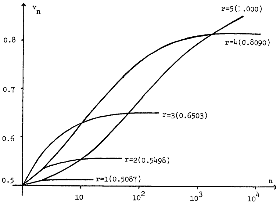
Figure 4.1. The graph of v_n for p -fold U(0,1) , p=5
