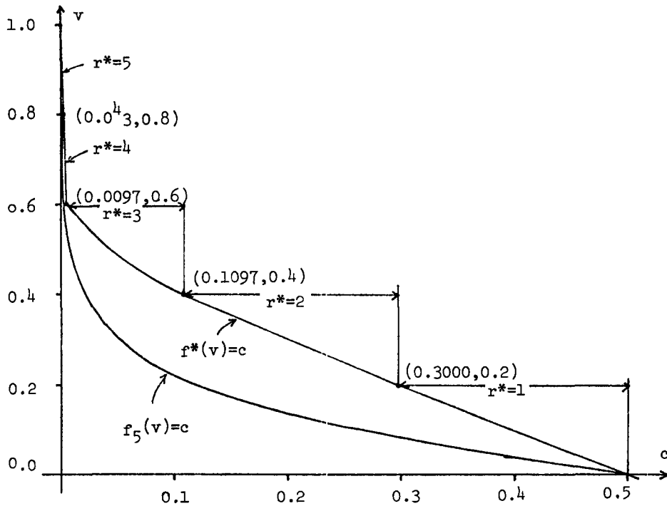
Figure 5.1. The majority level r^* for p=5
