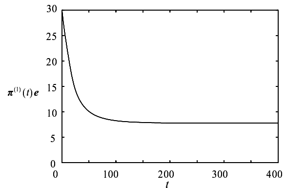
Figure 3: Mean queue length ( \rho/c = 0.7 )
